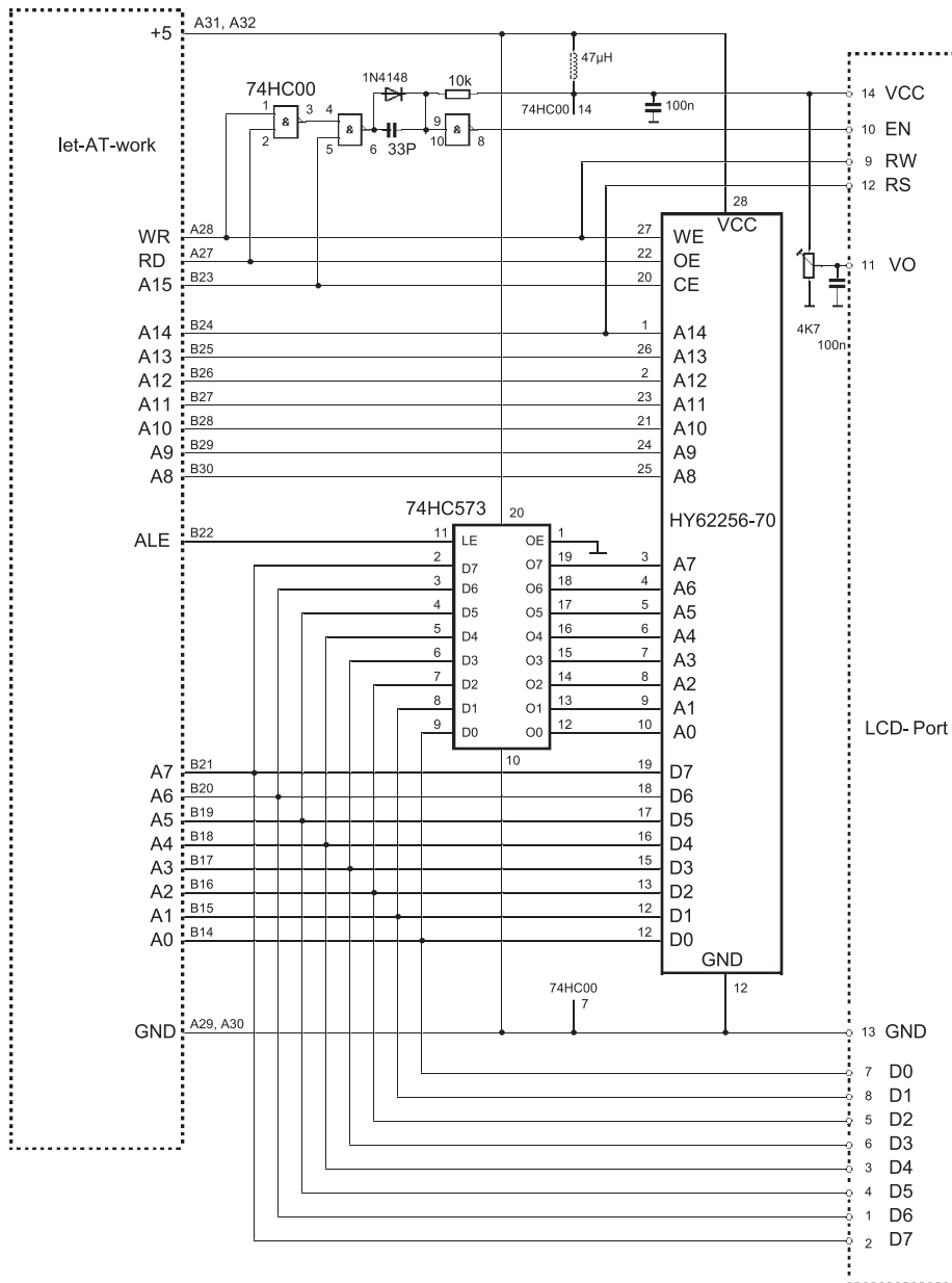
schematic for LCD/RAM module
