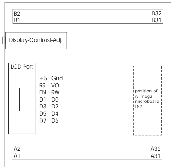
RAM/LCD module top view
